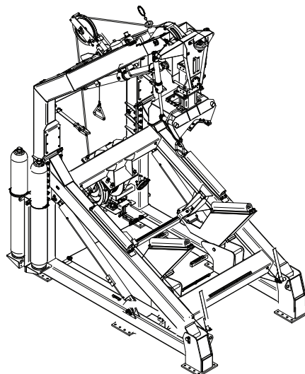
PRH 35A RESCUE BOAT DAVIT
